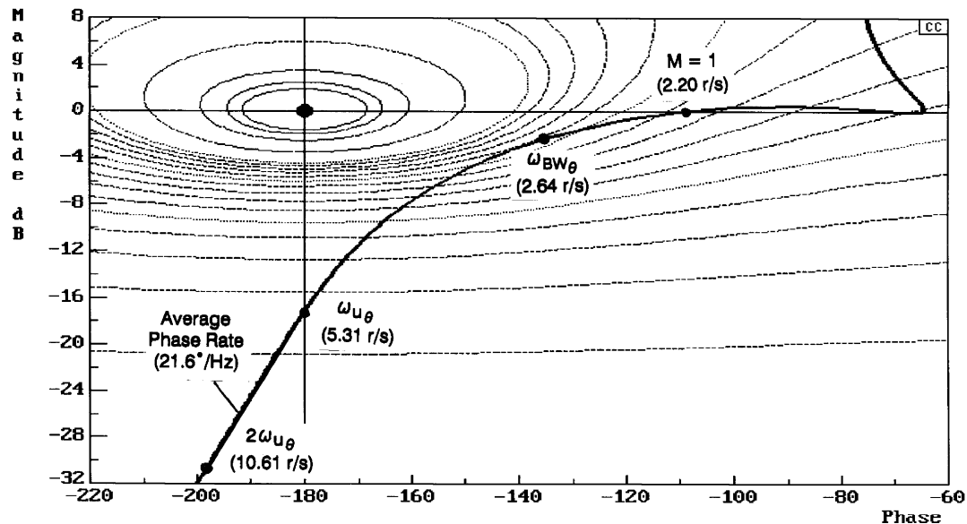
Fig. 8 X-15 pitch attitude frequency response at the flight 1-1-5 landing flare condition.
