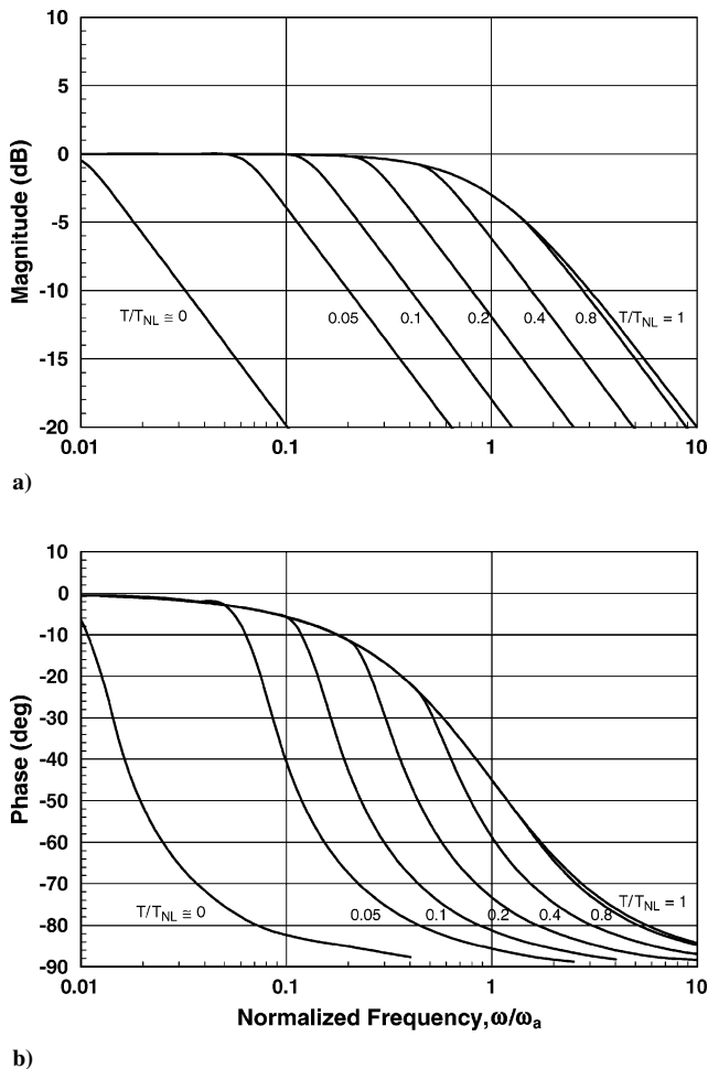
Fig. 3 Frequency response of simplified nonlinear actuator model.
