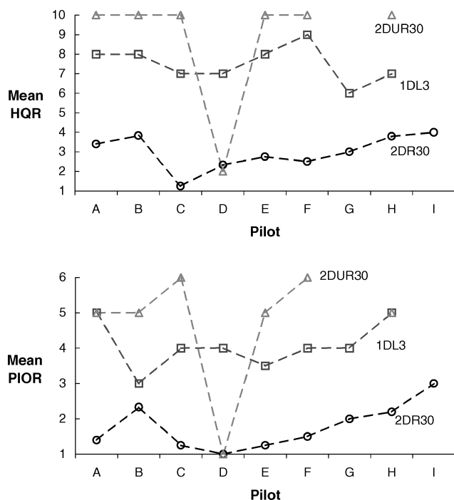
Fig. 15 Pilot rating variability (reproduced from Ref. 16).
