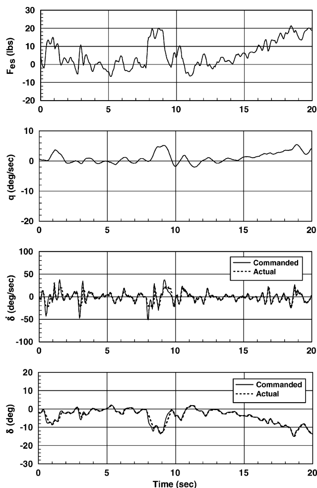
Fig. 11 Example time history segment for configuration 2P with 20-deg/s rate limit (tendency to PIO evidenced by phasing between stick force and pitch rate at t = 9 –13 s).
